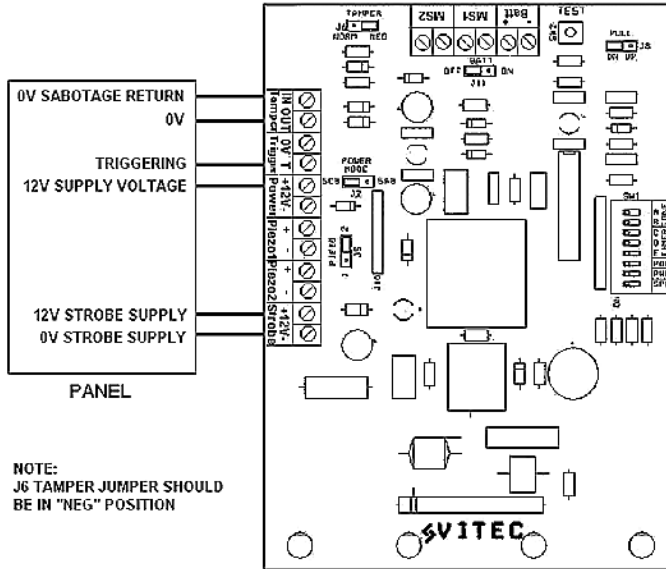
Example 2: Connection with is Alarm panel
