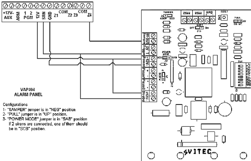
Example 2: Connection with is Alarm panel
