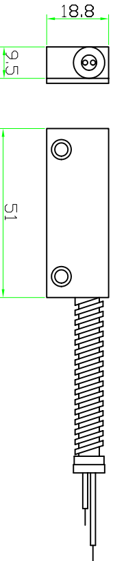
magnet
